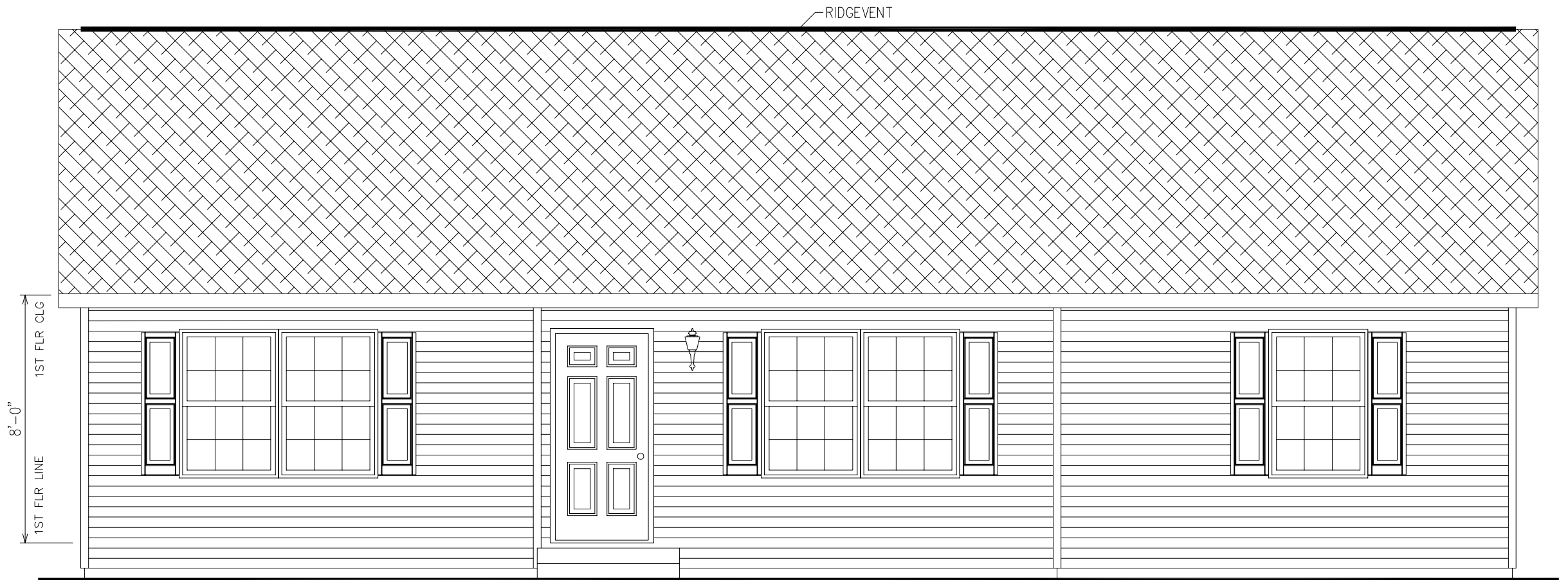
FRONT ELEVATION
