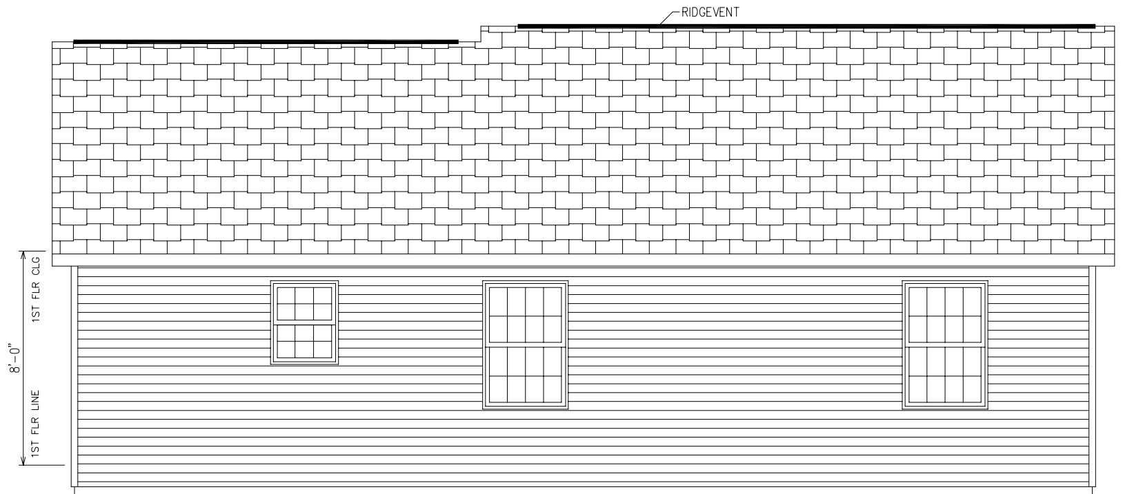
REAR ELEVATION
