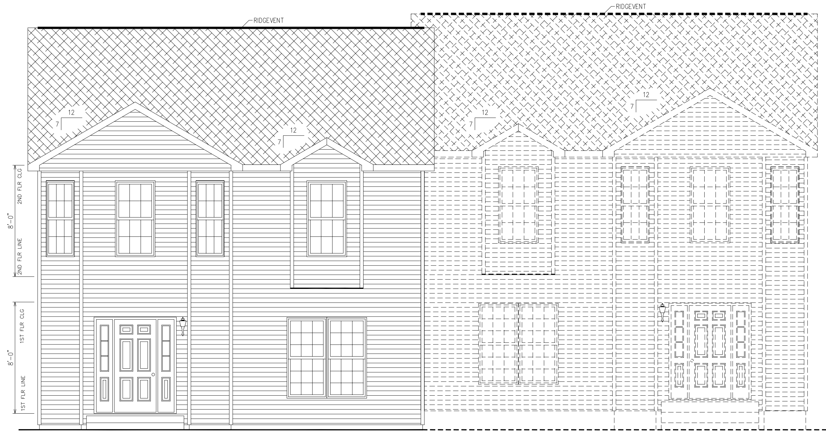
FRONT ELEVATION
